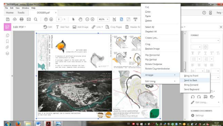
Screenshot 10
