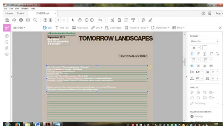
Screenshot 11
