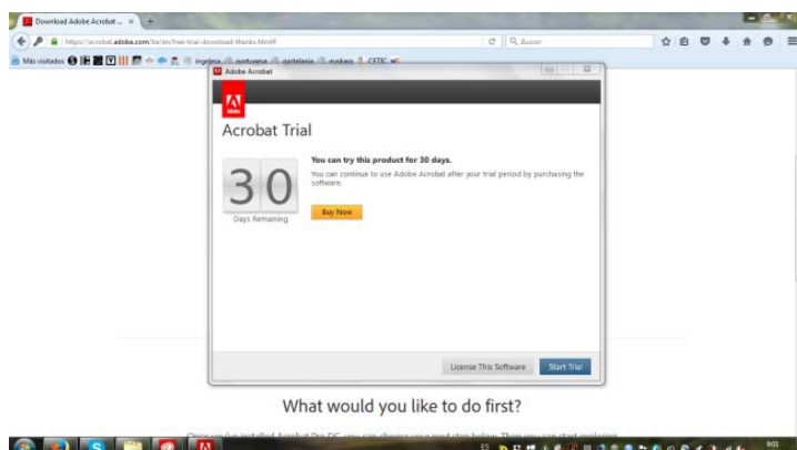
Screenshot 6
