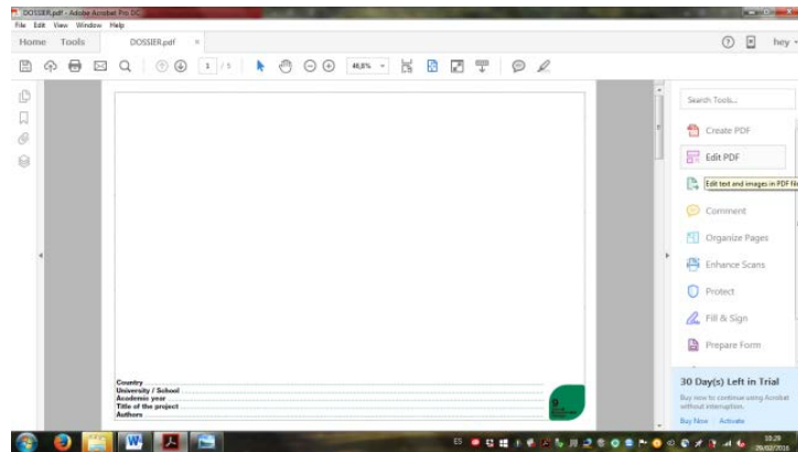
Screenshot 7
